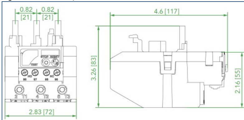
Figure 5 - Overloads, NR2-93G series
